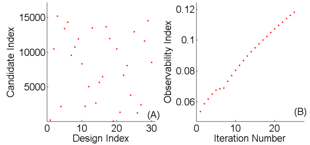
Fig. 5. (A) The selected poses for the optimal design based on the OI . (B) The observability index ( OI ) for each pose selection iteration.
