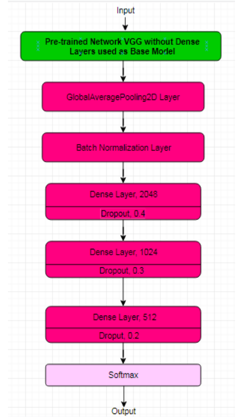
Figure 5. Architecture of Proposed Model built on VGG-19
